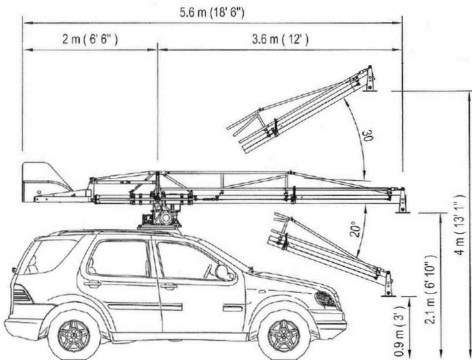
Scorpio Arm 12' Configuration on Mercedes ML63
