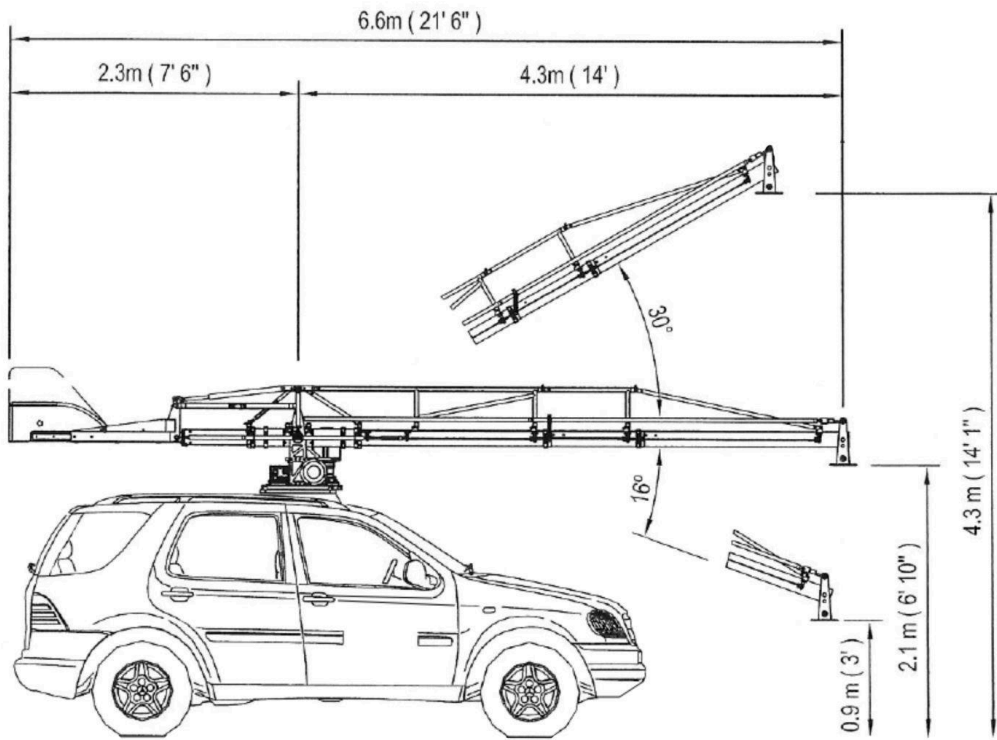
Scorpio Arm 14' Configuration on Mercedes ML63
